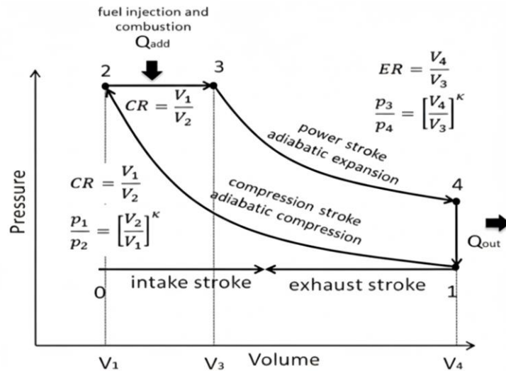
Fig 12.1 Pressure-Volume Diagram of Diesel cycle
