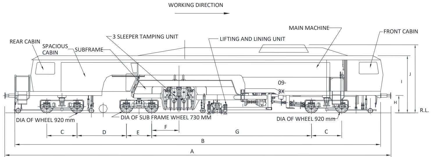
TAMPING EXPRESS
